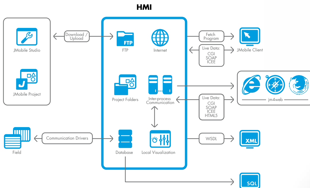
The modular JMobile architecture: cross-platform operation, monitoring and control almost anywhere at anytime
